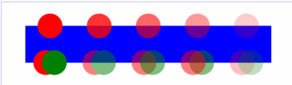
Example opacity01
