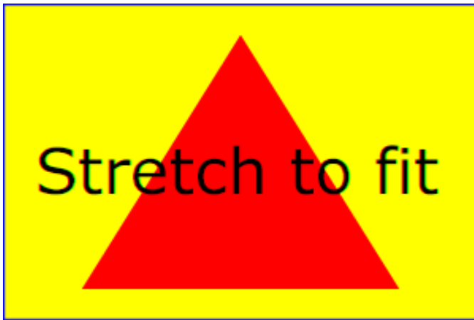
Example viewBox
