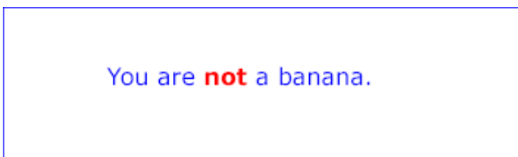
Example tspan01
